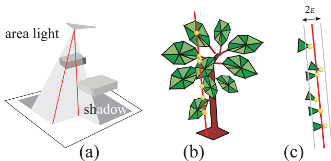
Figure 2: (a) Shadow boundaries are delimited by extremal stabbing lines (in red). (b) In complex models, stabbing lines may contain multiple collinear vertices. (c) If vertices are almost collinear, we choose to consider them as being on the same line.
